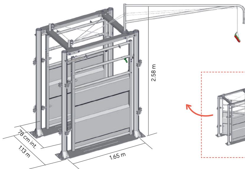
CO3050 Sorting gate on platform
